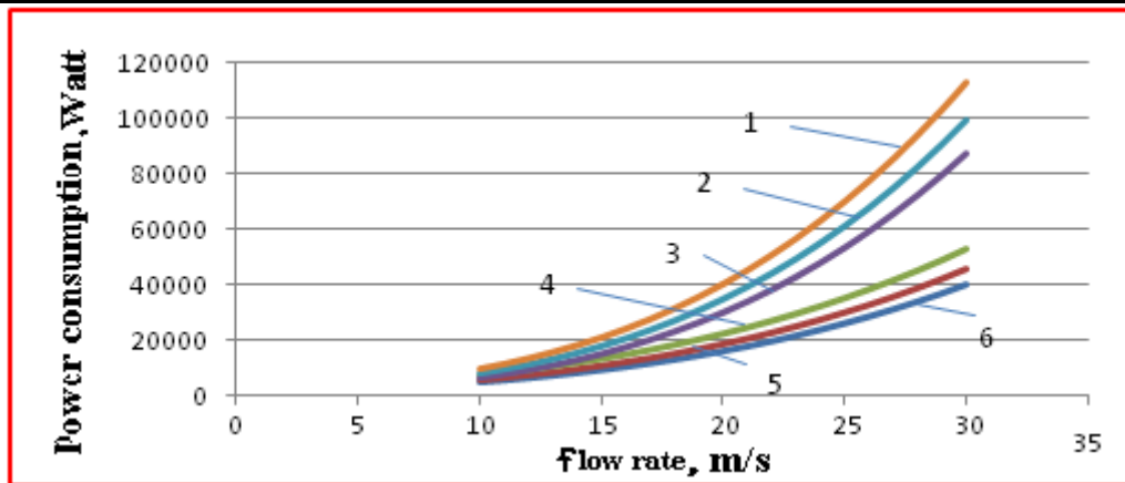
Fig.1. power consumption depending on the type, flow rate, and pipeline parameters.
