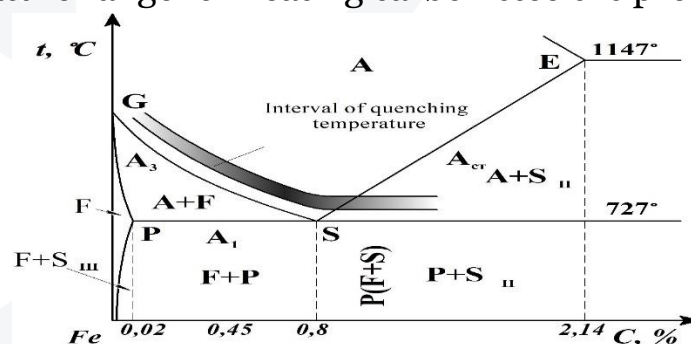
Figure 3. Optimum heating temperature range for quenching carbon steels
