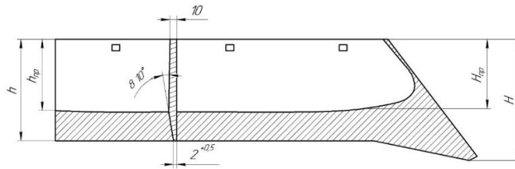
Figure 1. Structural and boundary dimensions of Lemex
